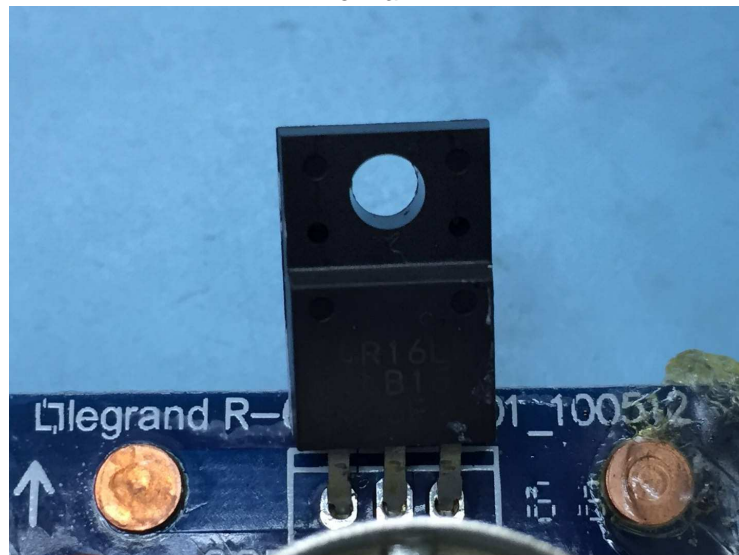
Triac
