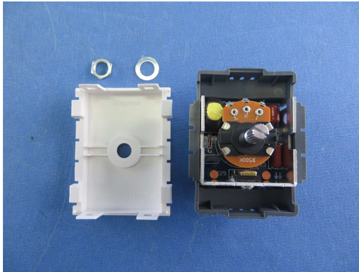
Cover opened
