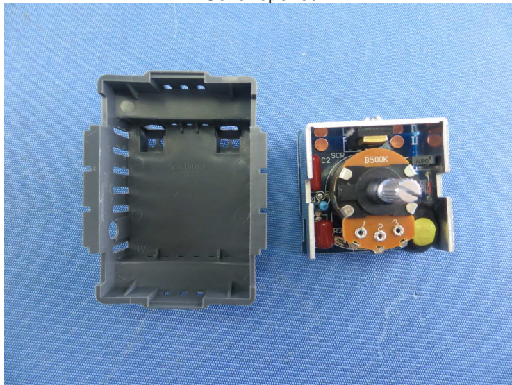
Bottom box removed
