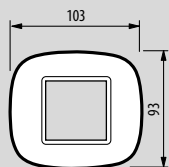
Plaque 2 modules
