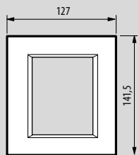
Plaque 3+3 modules
