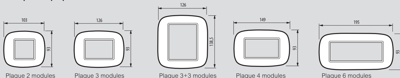
Plaque 2 modules
