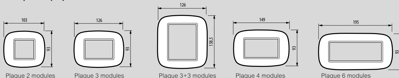
Plaque 2 modules
