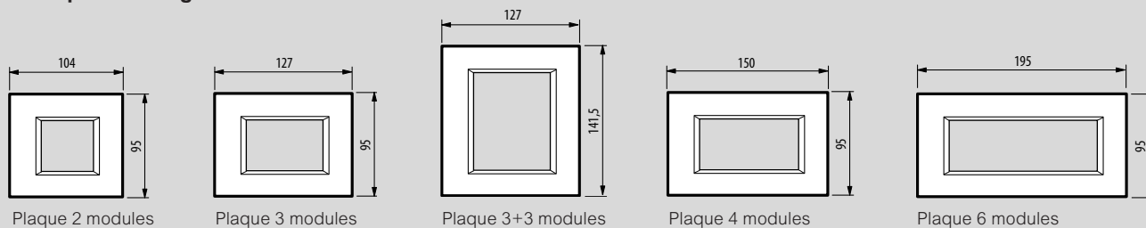
Plaque 2 modules
